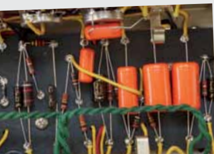
View inside: Blackface Tube Reverb Kit.
