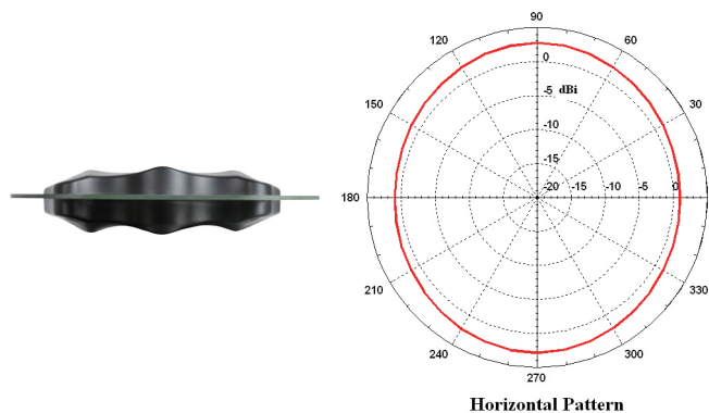
Figure 5: Horizontal pattern for AT-70Wa antenna.
