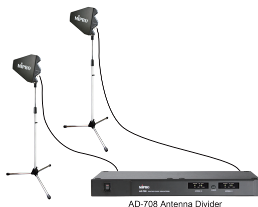
Figure 1: The system cable length does not exceed the limit of maximum acceptable line signal loss. (Connected to RX Only connector of the antenna)
