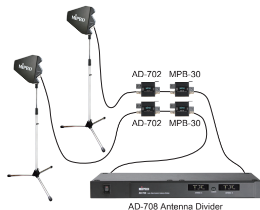
Figure 2: The system cable length exceeds the maximum length of adequate limit. (Connected to RX Only connector of the antenna)
