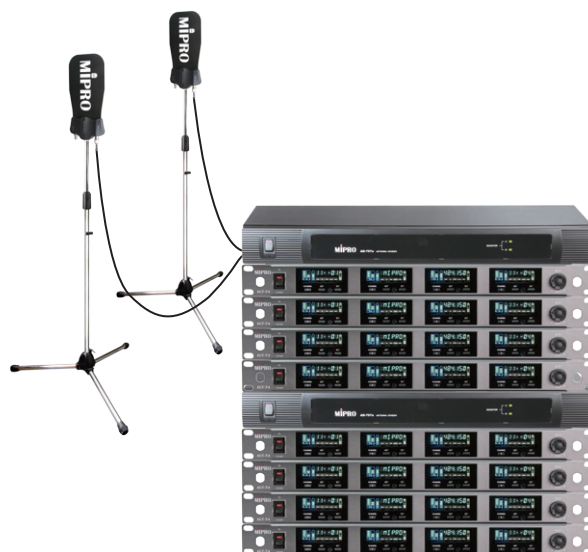
Figure 11: Two AD-707a wideband antenna dividers with eight quad-channel receivers to form a 32-channel system.
