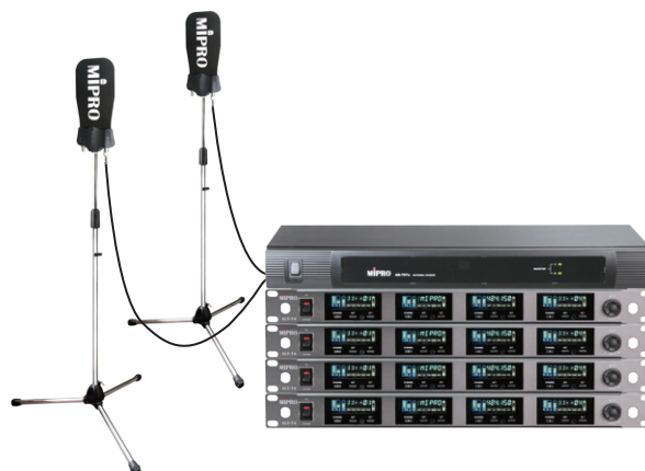
Figure 10B: Four MIPRO ACT-74 quad-channel receivers installed with an AD-707a wideband antenna divider.
